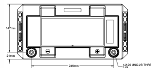
ODS-AGM70 RIGHT POSITIVE FEMALE TERMINALS
